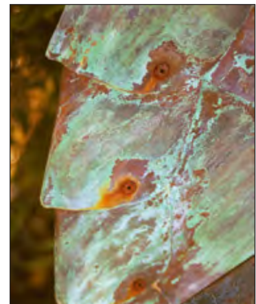
Figure III-10. Steel rivets used to join sections of exposed copper sheet create an ideal opportunity for galvanic corrosion. In this case, less noble steel corrodes while more noble copper remains protected. Corrosion is accelerated by large differences in area size between the two metals.
